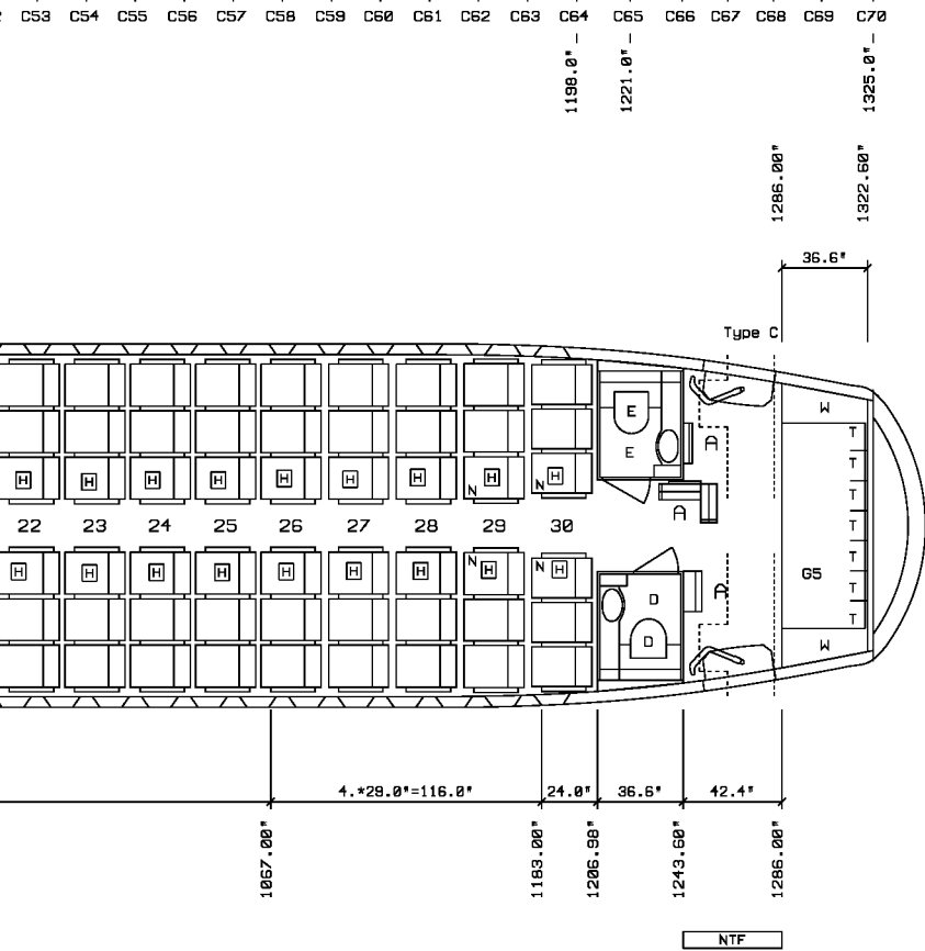
6 ABREAST CONSTANT SECTION
